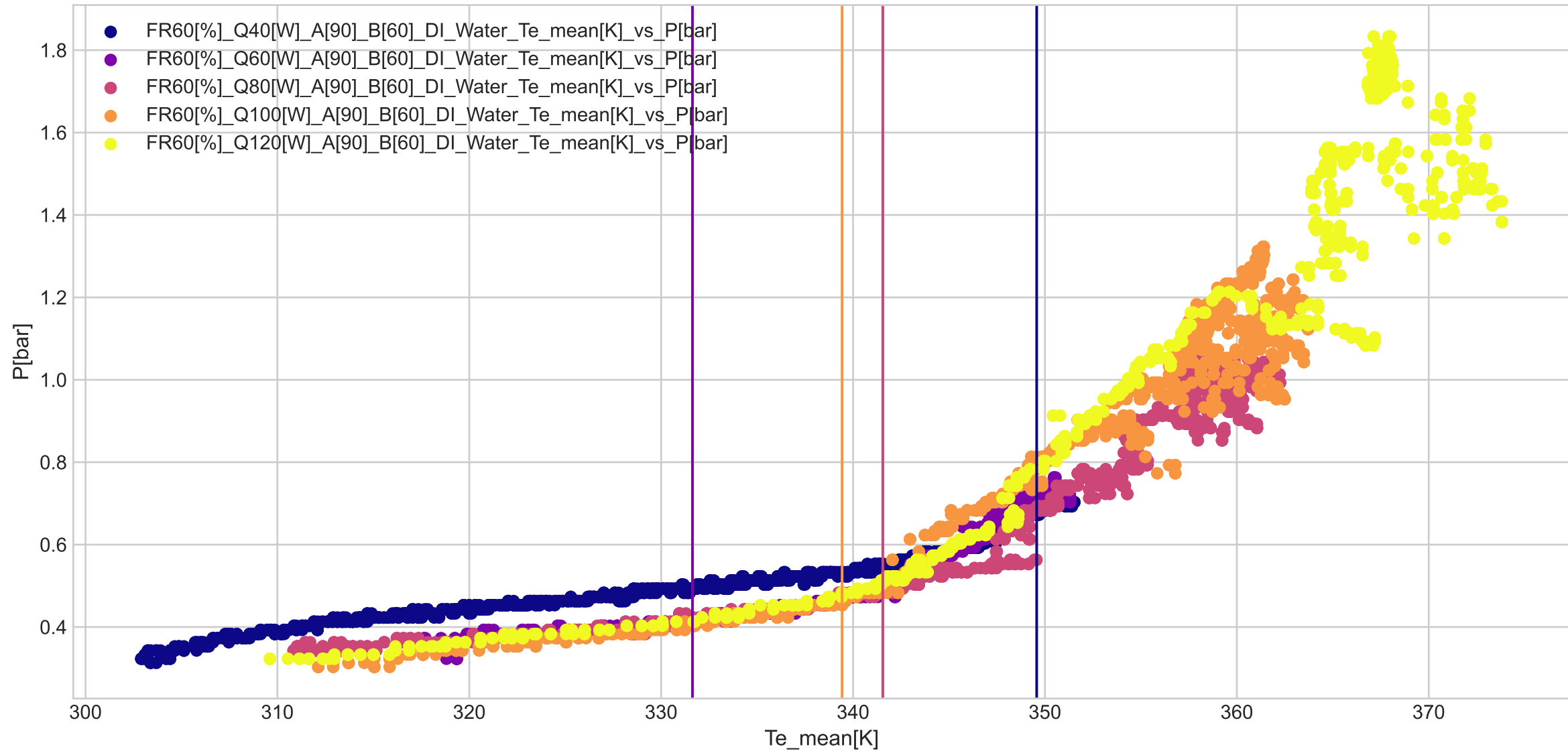
FR [60]% - Q [ 40 60 80 100 120]W - alpha [90] - beta [60] - DI_Water
